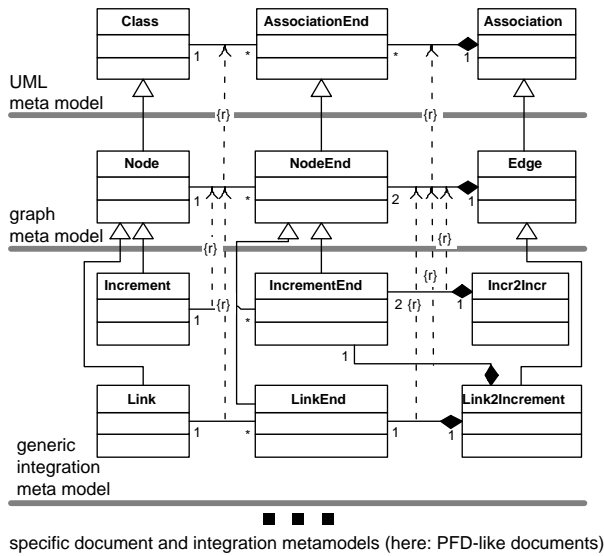
Fig. 14 Extension of the UML meta model
