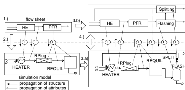
Fig. 2 Integration between flowsheet and simulation model
