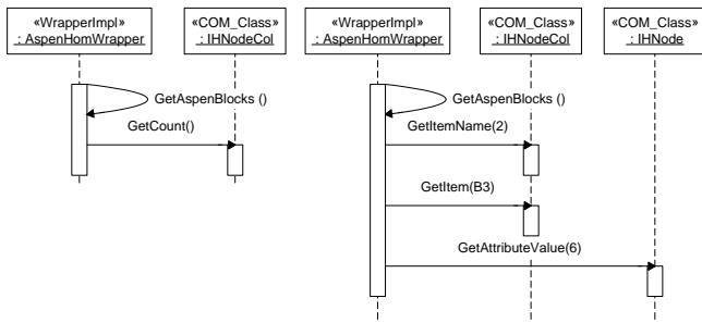
Fig. 10 Specification of operation NumberOfBlocks (left sequence diagram) and of operation GetAspenBlockType (right sequence diagram)
