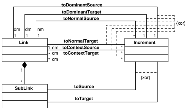
Fig. 12 Structure of links
