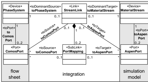
Fig. 15 Link type definition
