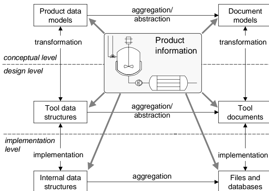
Fig. 2: Different perspectives on an integrated information model for the representation of design process information.
